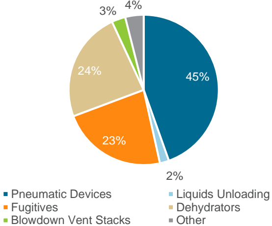
Methane Contribution
