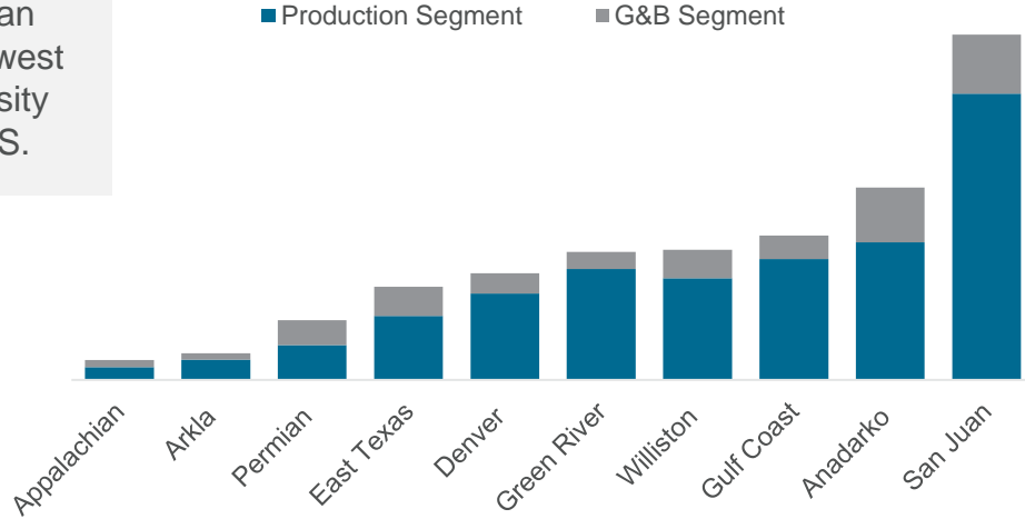
Methane Contribution
